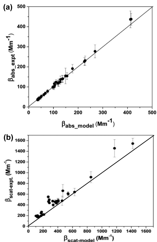
Figure 3. (a) Comparison of \beta_{\text{abs}} obtained from experiment and model calculations. (b) Comparison of \beta_{\text{scat}} obtained from experiment and model calculations.
