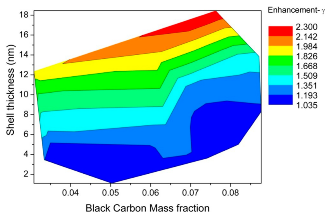
Figure 4. Absorption enhancement as a function of BC mass fraction and shell thickness. Each color shows range of absorption enhancement.
