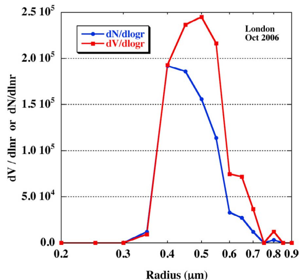
Figure 4. In situ measured ambient aerosol sizes associated with a fog event in London from Dall'Osto et al. [2009] (with additional conversion to volume distribution). These large submicron particles are composed of hydroxymethanesulphonate, which is a chemical species that is only formed in aqueous phase chemistry and therefore a tracer for aerosol processing by cloud or fog.
