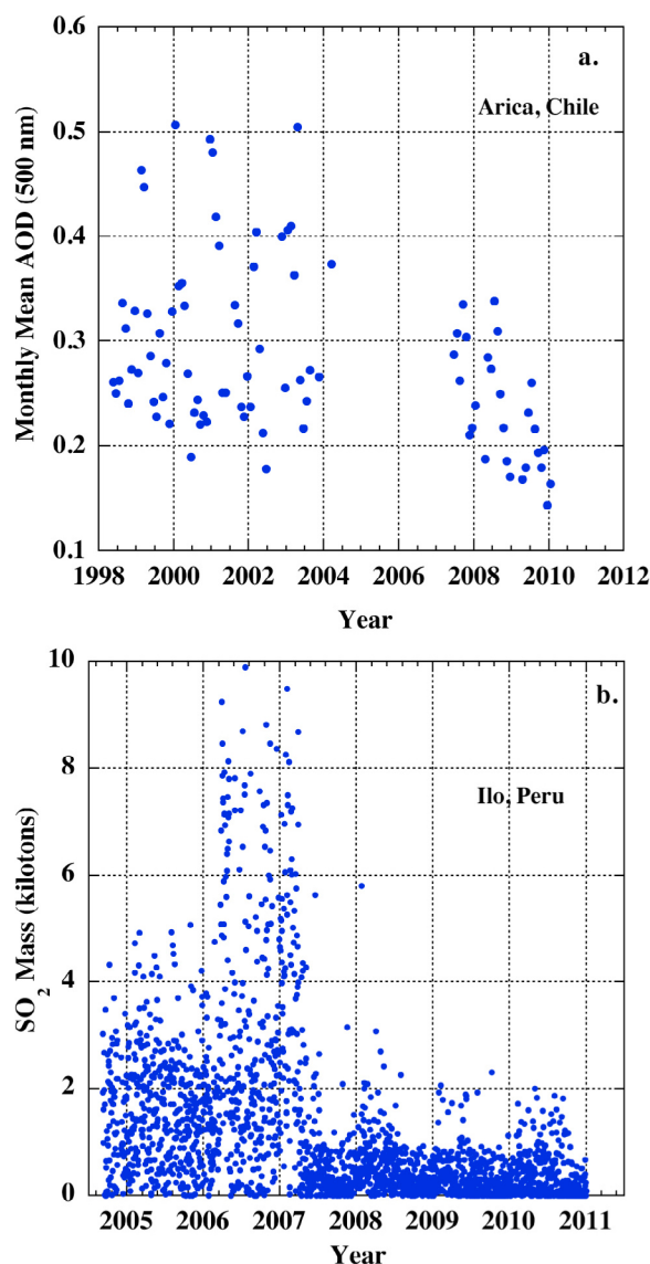
Figure 10. (a) Time series of the AERONET-measured monthly mean AOD (500 nm) at Arica, Chile, from 1998 to 2010, with a gap in the data from April 2004 through May 2007. (b) Daily average SO 2 mass column amounts measured by the OMI satellite instrument at Ilo, Peru [Carn et al. , 2007], from September 2004 through 2010. Note that the highest total column SO 2 measured in 2006 through spring 2007 was due to the additional source of the Ubinas volcano eruptions upwind of Ilo.
