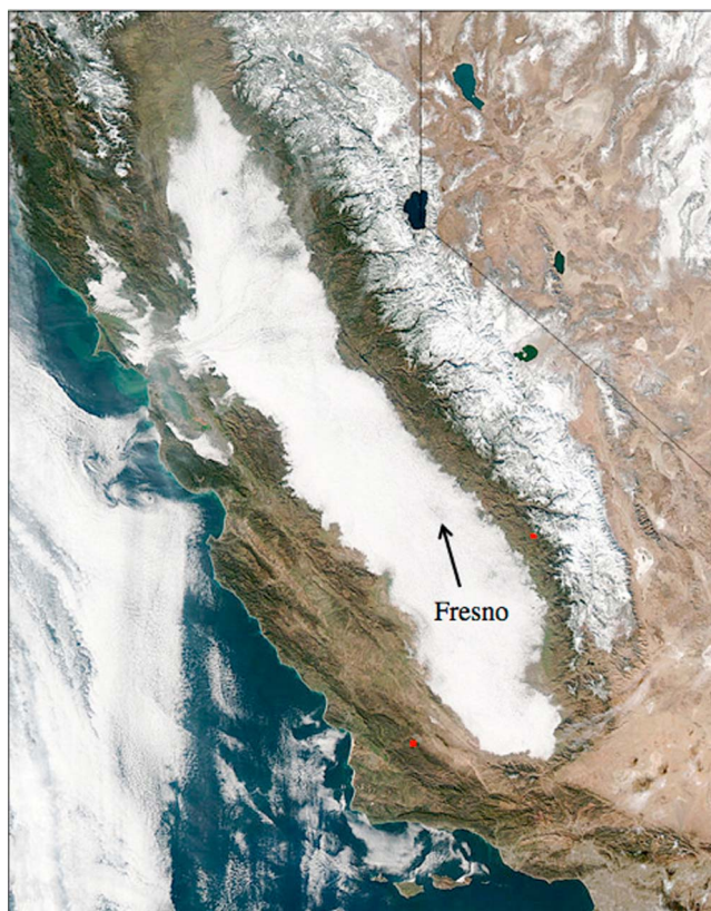
Figure 11. MODIS Aqua image from 13 January 2004 at 21:10 UTC showing extensive fog in the Central Valley of California; the location of Fresno is indicated. (Image courtesy of NASA/Goddard Space Flight Center Rapid Response.)
