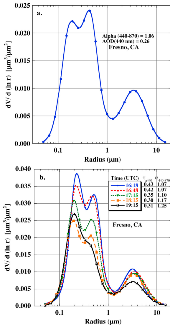
Figure 12. (a) Almucantar size distribution retrieval made at 23:32 UTC ( 75^\circ solar zenith) on 13 January 2004 at Fresno from \sim 2.4 h after the MODIS image shown in Figure 11. (b) Size distribution retrievals from Fresno on the morning of 11 February 2006 over a time interval of \sim 3 h for these five almucantar scans.
