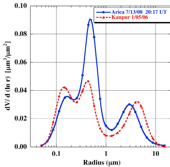
Figure 7. Almucantar retrieval made at Arica, Chile, on 13 July 2008 after the dissipation of the stratocumulus layer over the site. The 440 nm AOD during the almucantar scan averaged 0.58, and the \alpha_{440-870} was 0.77. Similar to the size distribution retrievals at Kanpur (from Figure 3), Figure 7 shows a bimodal submicron size distribution at Arica with the largest of the two modes having a volume radius peak of \sim 0.48 \mu\text{m} .
