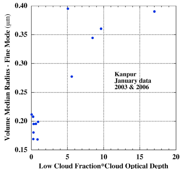
Figure 6. Product of low cloud fraction (cloud top pressure >600 mb) times low cloud optical depth from the MODIS cloud algorithm [Platnick et al. , 2003] at the Terra satellite overpass time (midmorning) at Kanpur versus the retrieved fine mode median radius (for January 2003 and 2006 only). The retrieved radius values are from almucantar scans made after the fog/low cloud had dissipated and are daily averages of all retrievals made in a given day.
